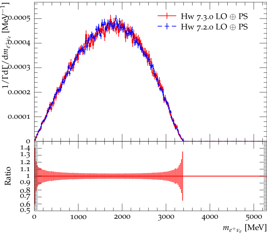
Mass of e^+ \nu_e in the decay B^+ \rightarrow \bar{D}^0 e^+ \nu_e
