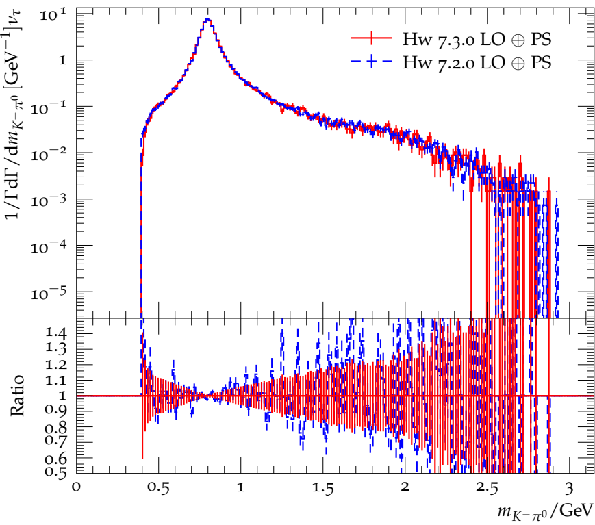
Mass distribution of the hadrons for \tau^- \rightarrow K^- \pi^0
