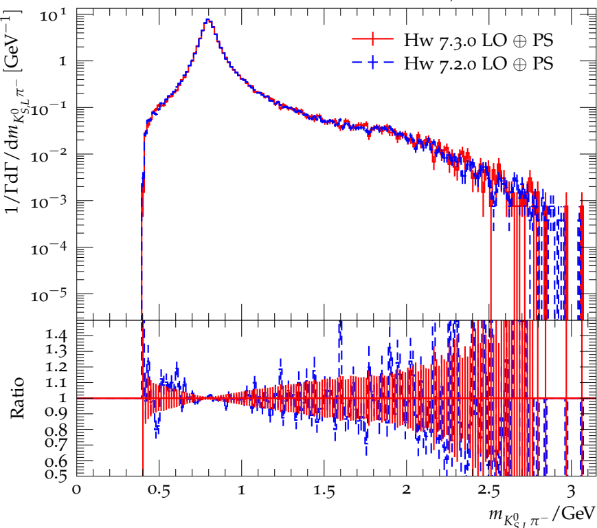
Mass distribution of the hadrons for \tau^- \rightarrow K_{S,L}^0 \pi^- \nu_\tau
