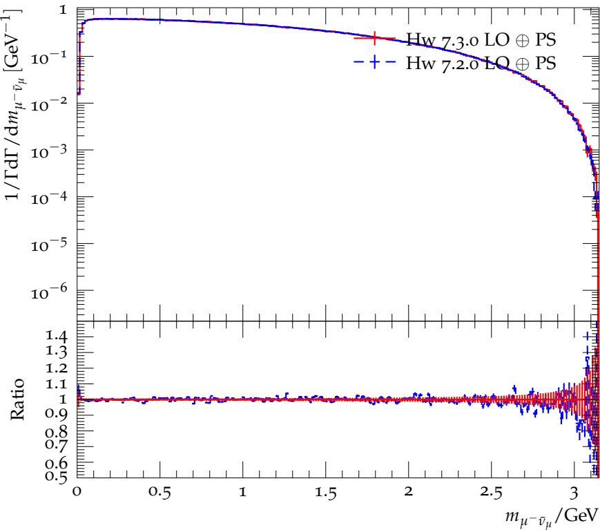
Mass distribution of the muon/neutrino for \tau^- \rightarrow \mu^- \bar{\nu}_\mu \nu_\tau
