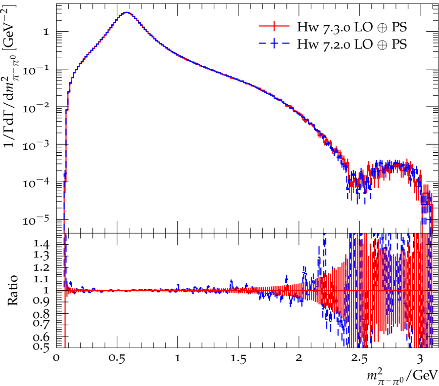
Mass distribution of the hadrons for \tau^- \rightarrow \pi^- \pi^0 \nu_\tau
