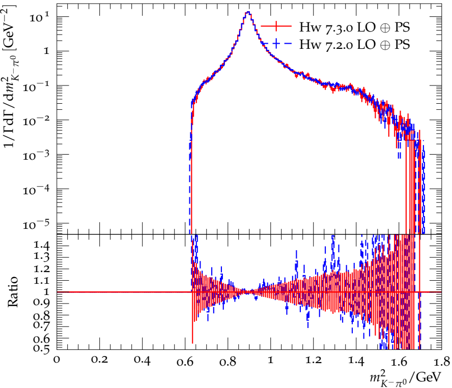
Mass distribution of the hadrons for \tau^- \rightarrow K^- \pi^0 \nu_\tau
