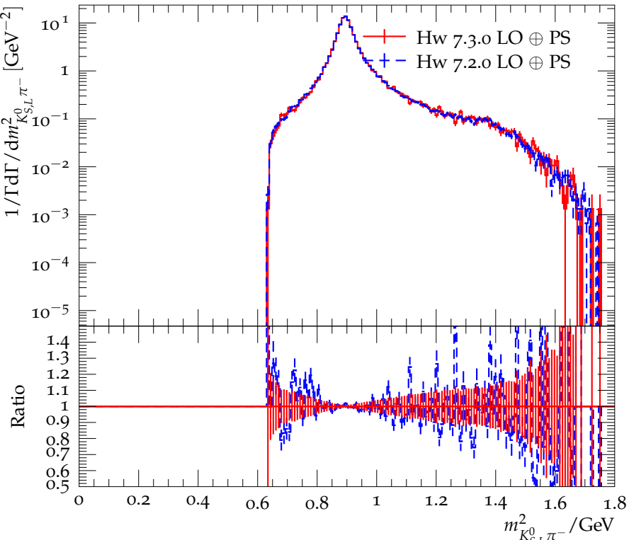
Mass distribution of the hadrons for \tau^- \rightarrow K_{S,L}^0 \pi^- \nu_\tau
