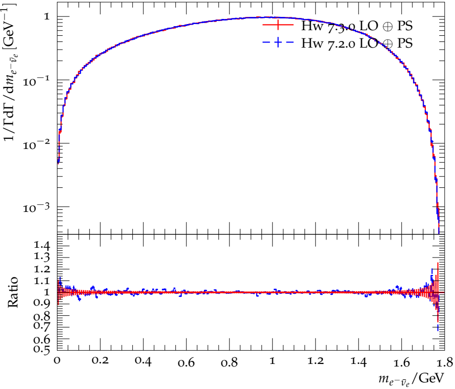
Mass distribution of the electron/neutrino for \tau^- \rightarrow e^- \bar{\nu}_e \nu_\tau
