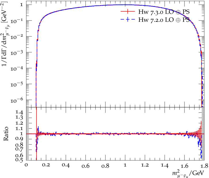
Mass distribution of the hadrons for \tau^- \rightarrow \mu^- \bar{\nu}_\mu \nu_\tau
