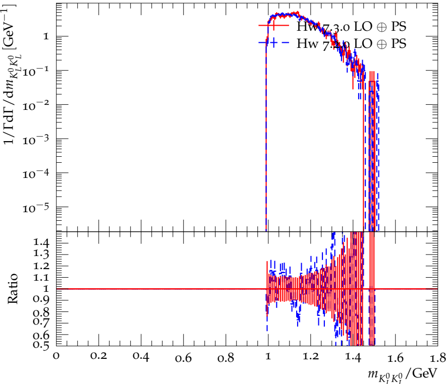
Distribution of the K_L^0 K_L^0 mass in \tau^- \rightarrow K_L^0 \pi^- K_L^0 \nu_\tau
