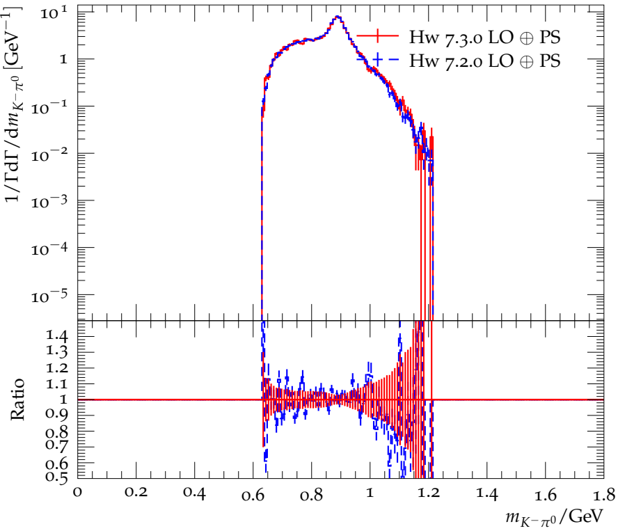
Distribution of the K^- \pi^0 mass in \tau^- \rightarrow K^- \pi^0 K^0 \nu_\tau
