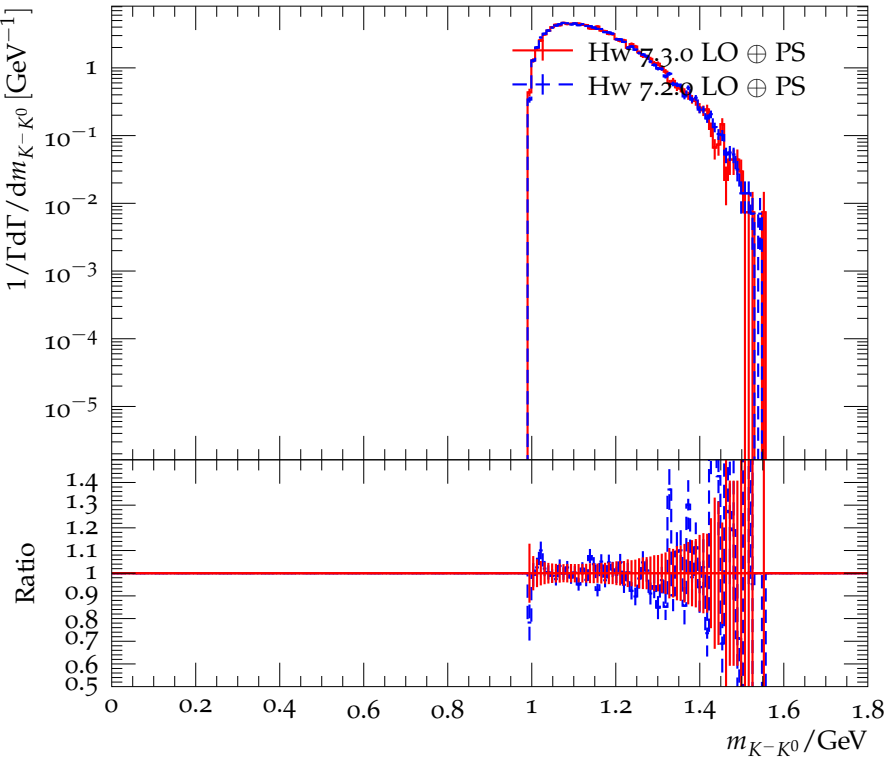
Distribution of the K^-K^0 mass in \tau^- \rightarrow K^- \pi^0 K^0 \nu_\tau
