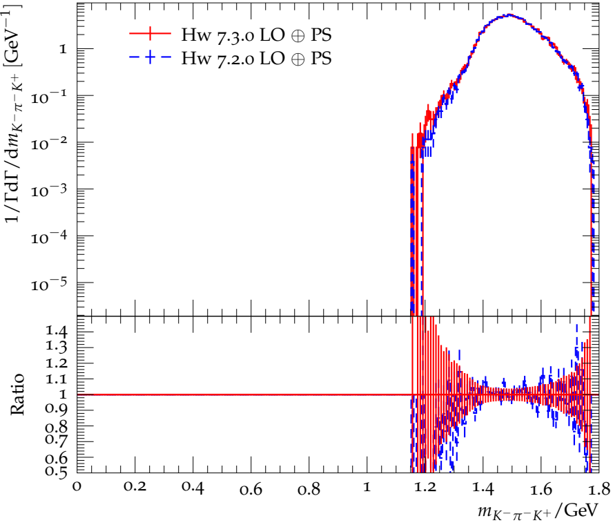
Distribution of the hadronic mass in \tau^- \rightarrow K^- \pi^- K^+ \nu_\tau
