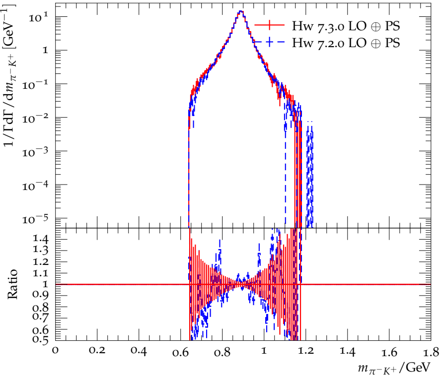
Distribution of the \pi^- K^+ mass in \tau^- \rightarrow K^- \pi^- K^+ \nu_\tau
