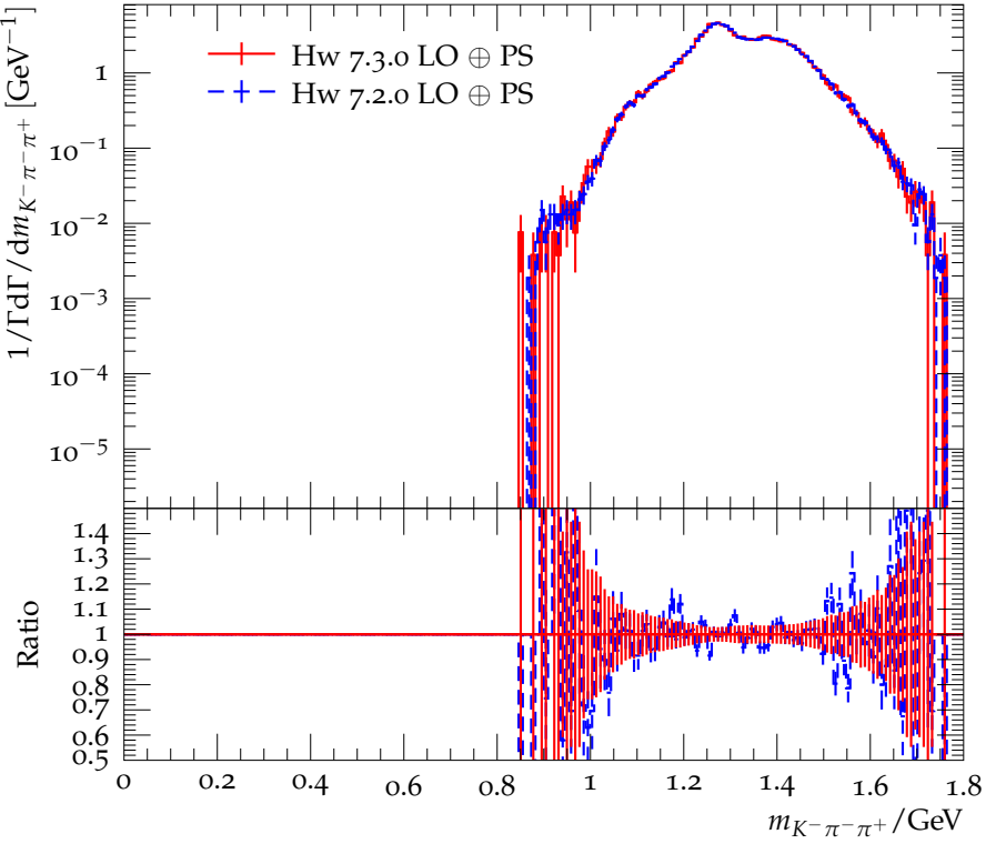
Distribution of the hadronic mass in \tau^- \rightarrow K^- \pi^- \pi^+ \nu_\tau
