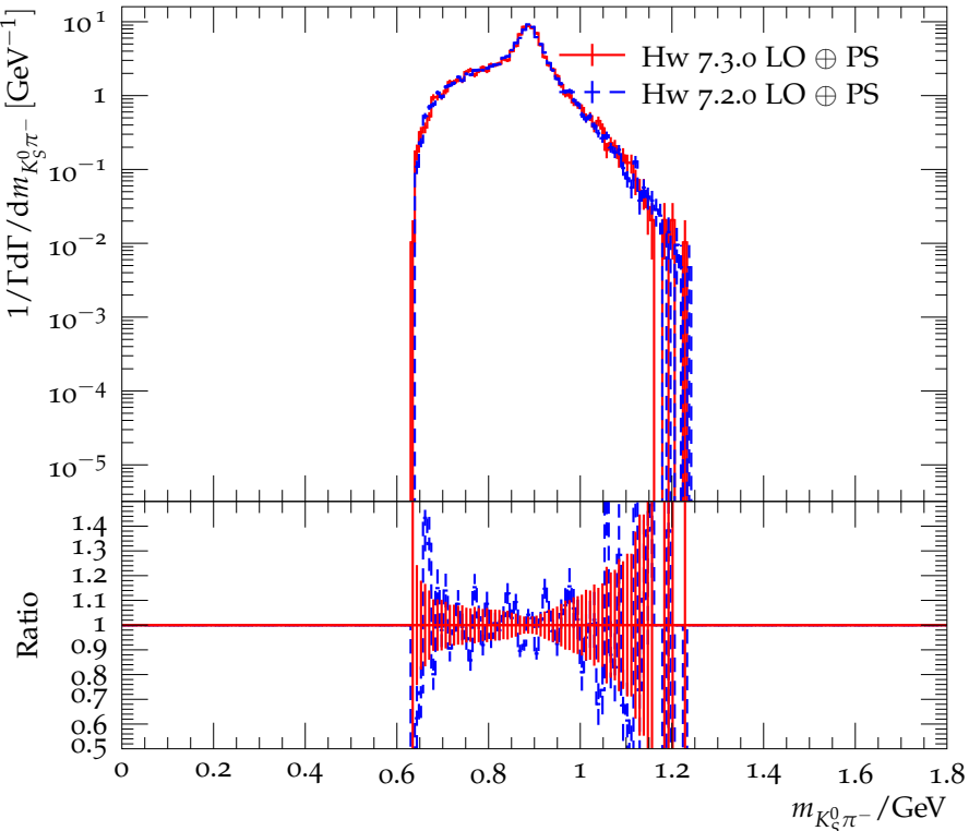
Distribution of the K_S^0\pi^- mass in \tau^- \rightarrow K_S^0\pi^- K_L^0\nu_\tau
