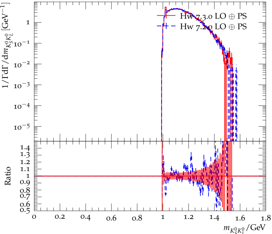
Distribution of the K_S^0 K_L^0 mass in \tau^- \rightarrow K_S^0 \pi^- K_L^0 \nu_\tau
