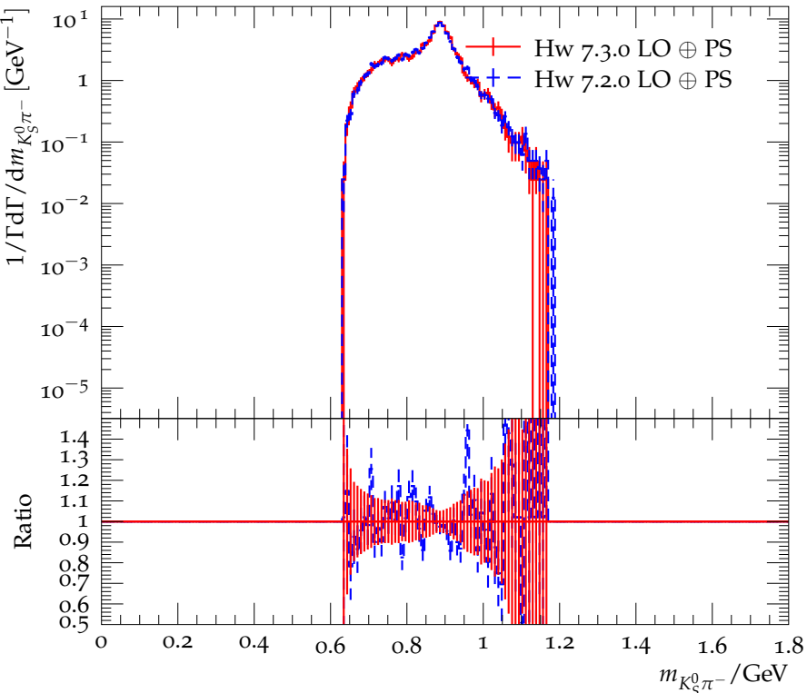
Distribution of the K_S^0\pi^- mass in \tau^- \rightarrow K_S^0\pi^- K_S^0\nu_\tau
