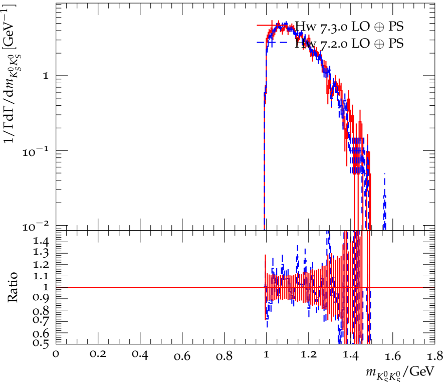
Distribution of the K_S^0 K_S^0 mass in \tau^- \rightarrow K_S^0 \pi^- K_S^0 \nu_\tau
