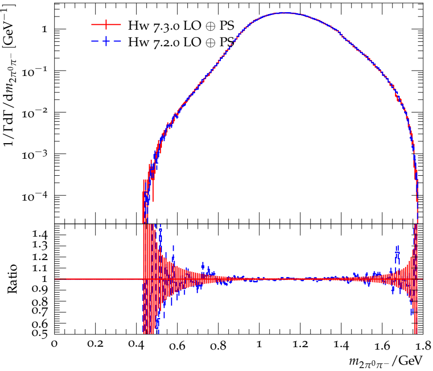
Distribution of the hadronic mass in \tau^- \rightarrow 2\pi^0\pi^-\nu_\tau
