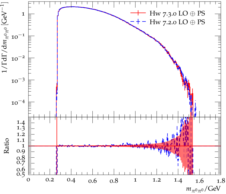
Distribution of the \pi^0\pi^0 mass in \tau^- \rightarrow 2\pi^0\pi^-\nu_\tau
