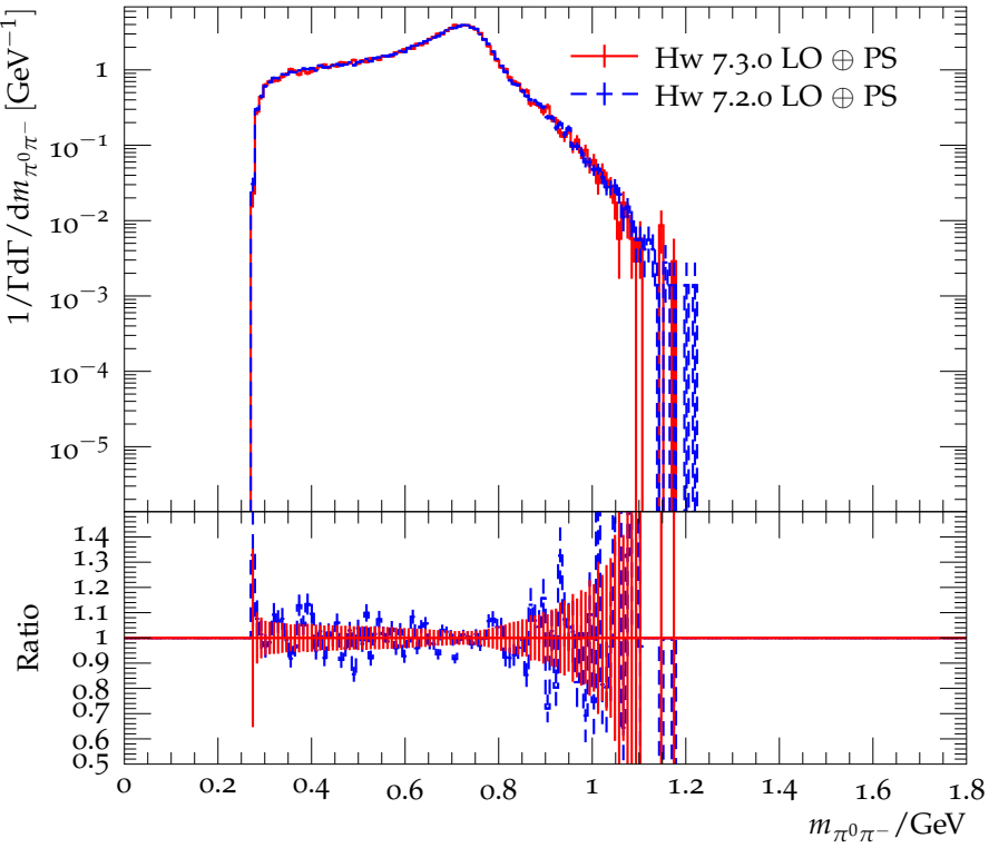
Distribution of the \pi^0\pi^- mass in \tau^- \rightarrow \pi^- \pi^0 \bar{K}^0 \nu_\tau
