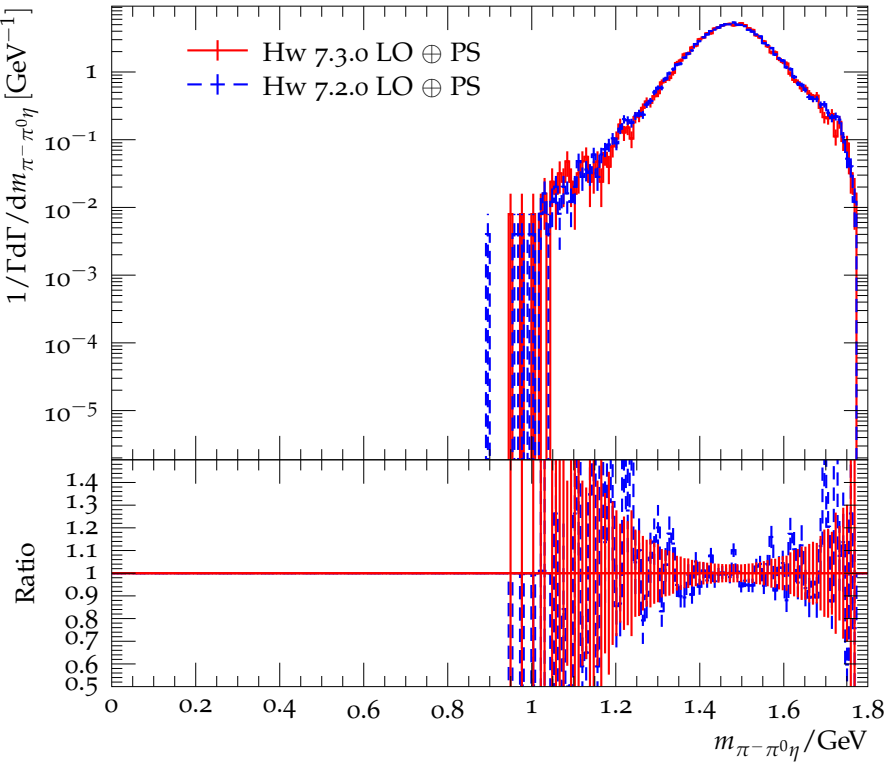
Distribution of the hadronic mass in \tau^- \rightarrow \pi^- \pi^0 \eta \nu_\tau
