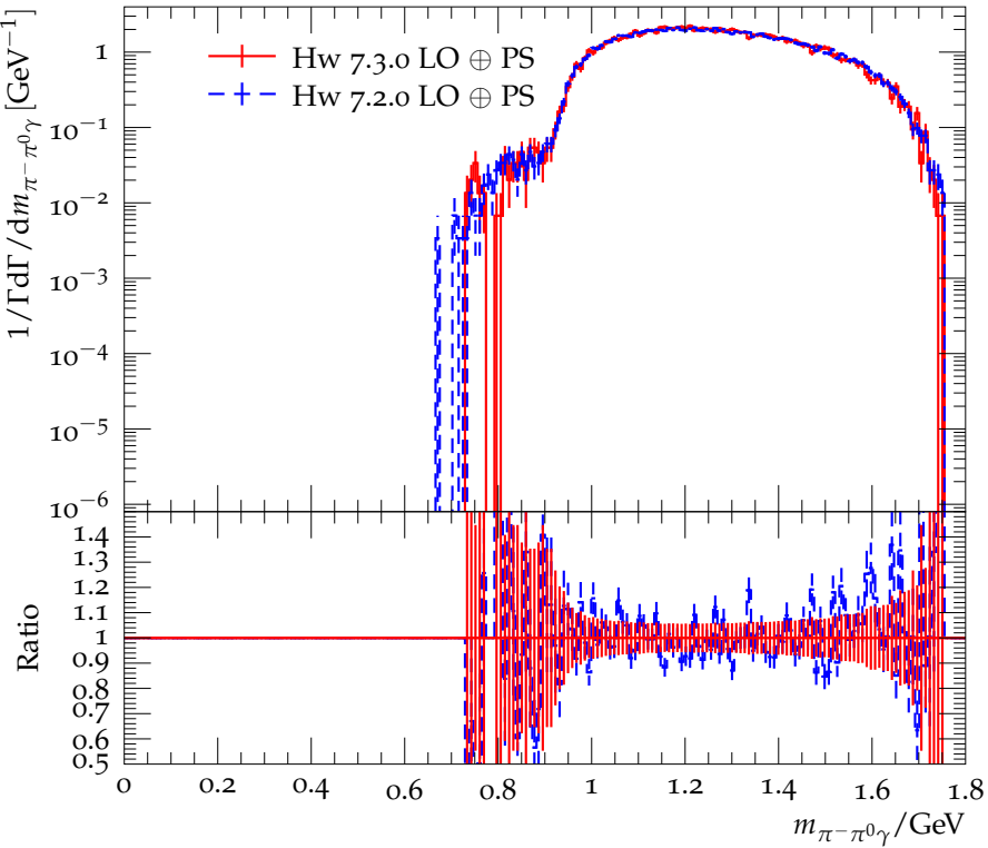
Distribution of the hadronic mass in \tau^- \rightarrow \pi^- \pi^0 \gamma \nu_\tau
