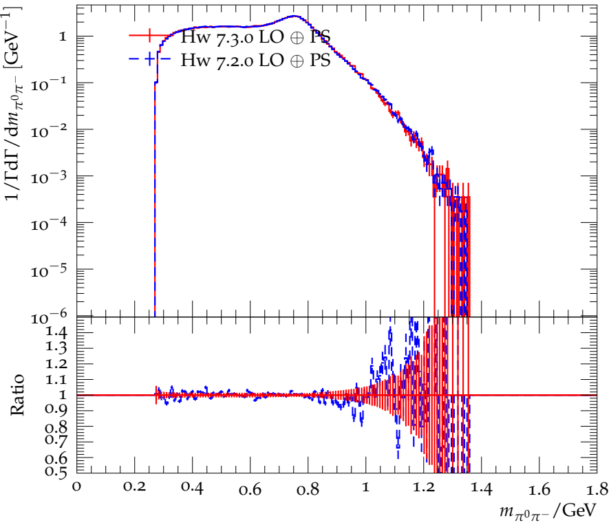
Distribution of the \pi^0\pi^- mass in \tau^- \rightarrow 3\pi^0\pi^-\nu_\tau
