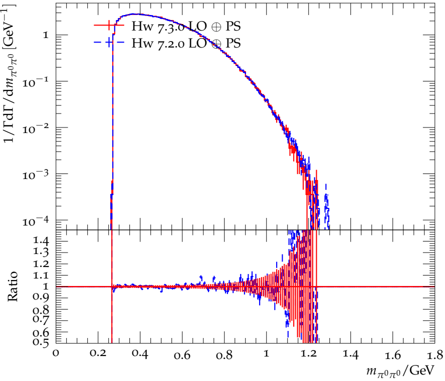
Distribution of the \pi^0\pi^0 mass in \tau^- \rightarrow 3\pi^0\pi^-\nu_\tau
