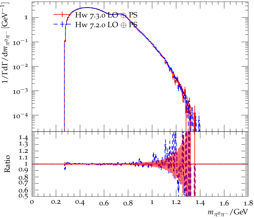
Distribution of the \pi^0\pi^- mass in \tau^- \rightarrow \pi^0\pi^+2\pi^-\nu_\tau
