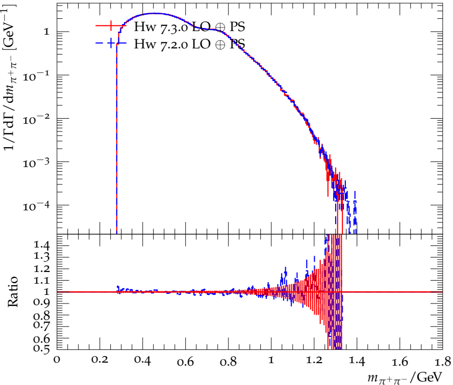
Distribution of the \pi^+\pi^- mass in \tau^- \rightarrow \pi^0\pi^+2\pi^-\nu_\tau
