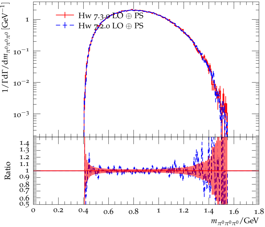
Distribution of the \pi^0\pi^0\pi^0 mass in \tau^- \rightarrow 3\pi^0\pi^-\nu_\tau
