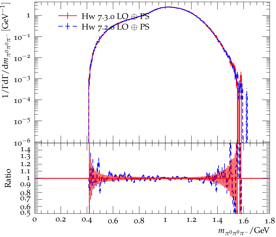
Distribution of the \pi^0\pi^0\pi^- mass in \tau^- \rightarrow 3\pi^0\pi^-\nu_\tau
