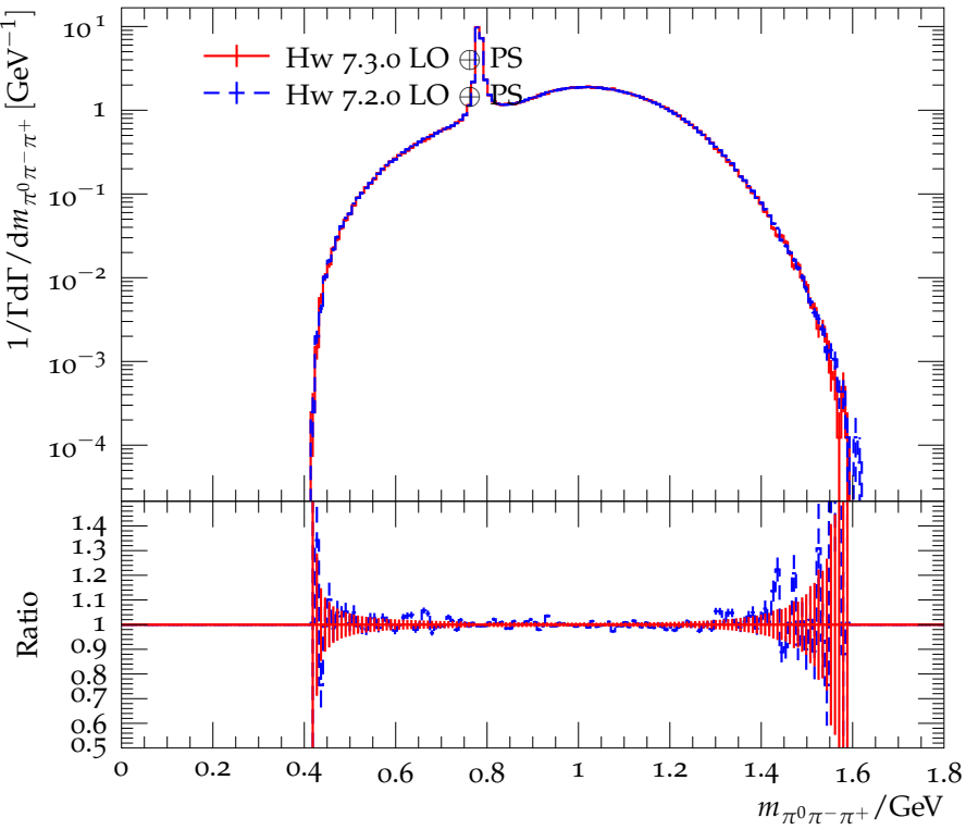
Distribution of the \pi^0\pi^-\pi^+ mass in \tau^- \rightarrow \pi^0\pi^+2\pi^-\nu_\tau
