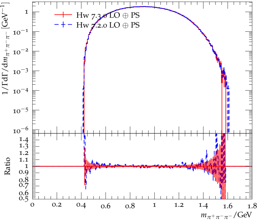
Distribution of the \pi^+\pi^-\pi^- mass in \tau^- \rightarrow \pi^0\pi^+2\pi^-\nu_\tau
