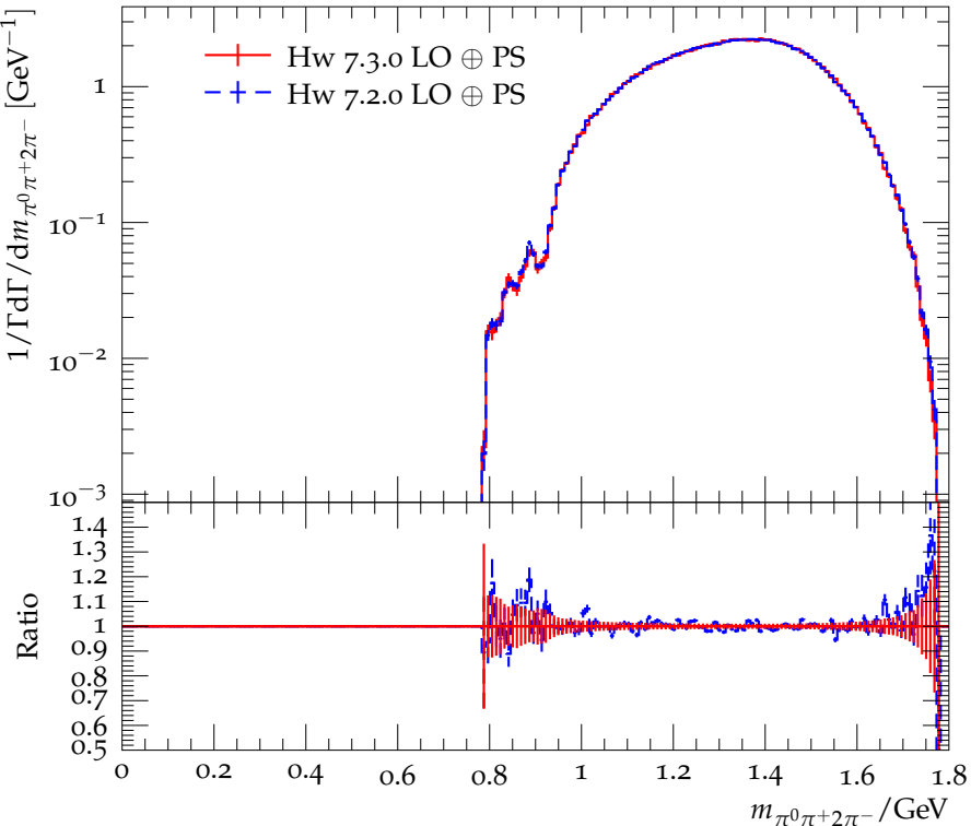
Distribution of the \pi^0\pi^+2\pi^- mass in \tau^- \rightarrow \pi^0\pi^+2\pi^-\nu_\tau
