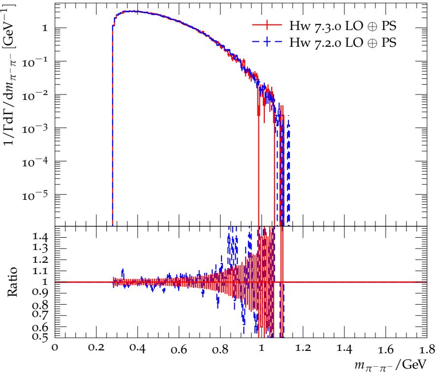
Distribution of the \pi^-\pi^- mass for \tau^- \rightarrow 2\pi^0 2\pi^-\pi^+\nu_\tau
