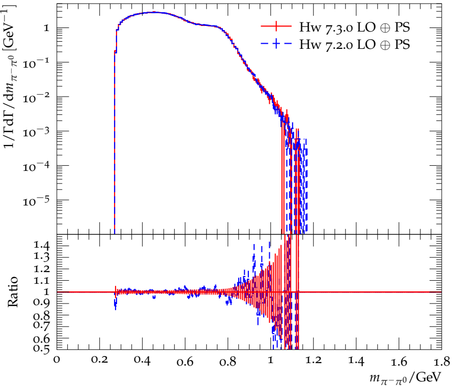
Distribution of the \pi^- \pi^0 mass for \tau^- \rightarrow 2\pi^0 2\pi^- \pi^+ \nu_\tau
