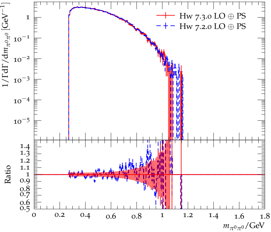
Distribution of the \pi^0\pi^0 mass for \tau^- \rightarrow 2\pi^0 2\pi^- \pi^+ \nu_\tau
