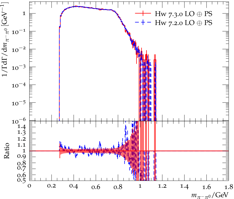
Distribution of the \pi^- \pi^0 mass for \tau^- \rightarrow 4\pi^0 \pi^- \nu_\tau
