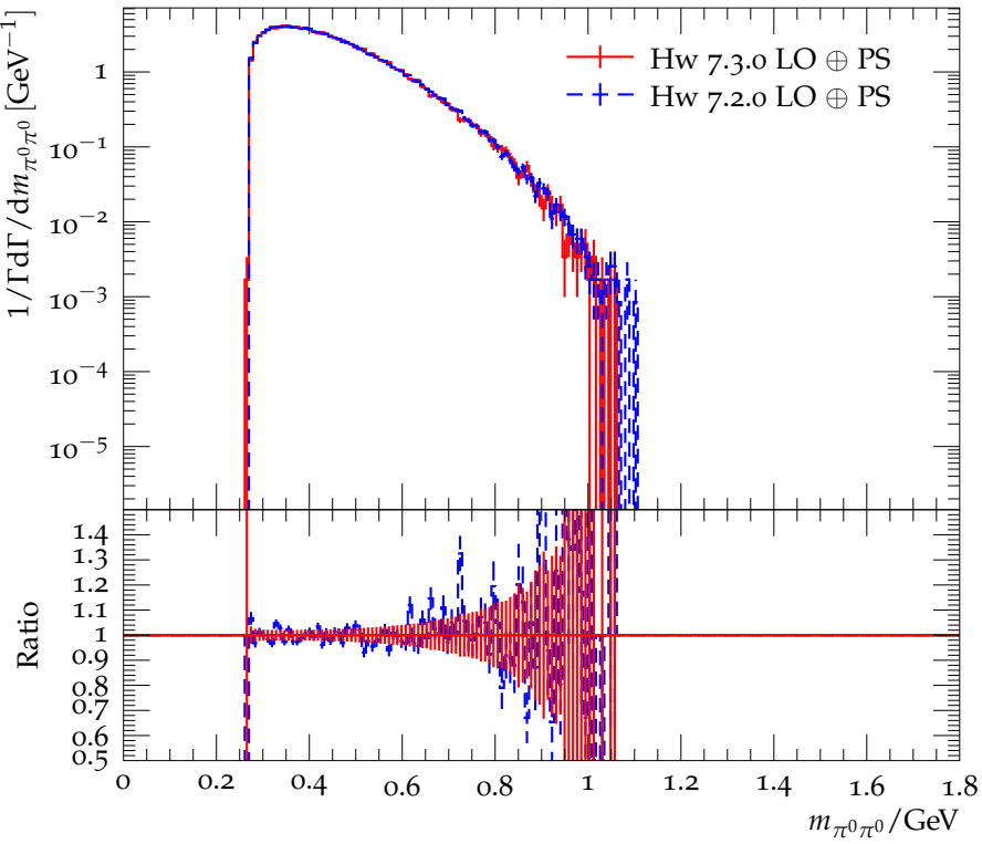
Distribution of the \pi^0\pi^0 mass for \tau^- \rightarrow 4\pi^0\pi^-\nu_\tau
