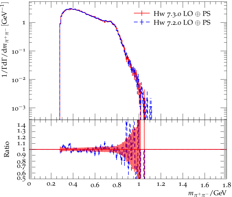
Distribution of the \pi^+\pi^- mass for \tau^- \rightarrow 3\pi^- 2\pi^+ \nu_\tau
