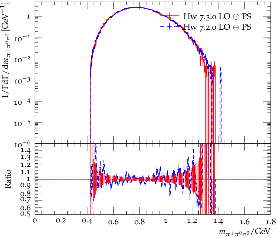
Distribution of the \pi^+\pi^0\pi^0 mass for \tau^- \rightarrow 2\pi^0 2\pi^- \pi^+ \nu_\tau
