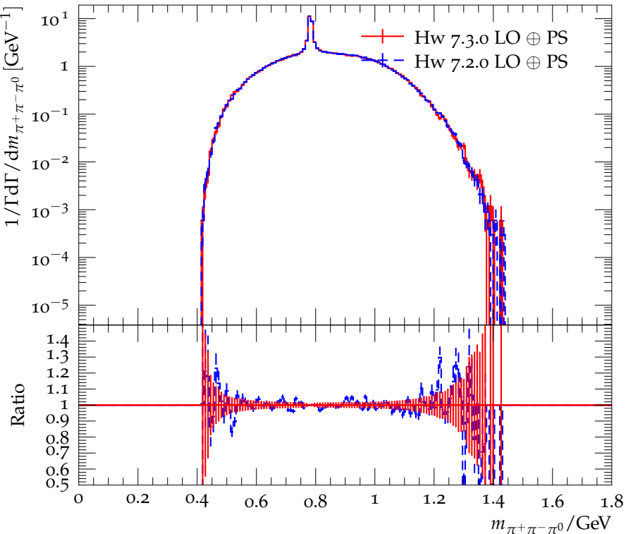
Distribution of the \pi^+\pi^-\pi^0 mass for \tau^- \rightarrow 2\pi^0 2\pi^-\pi^+\nu_\tau
