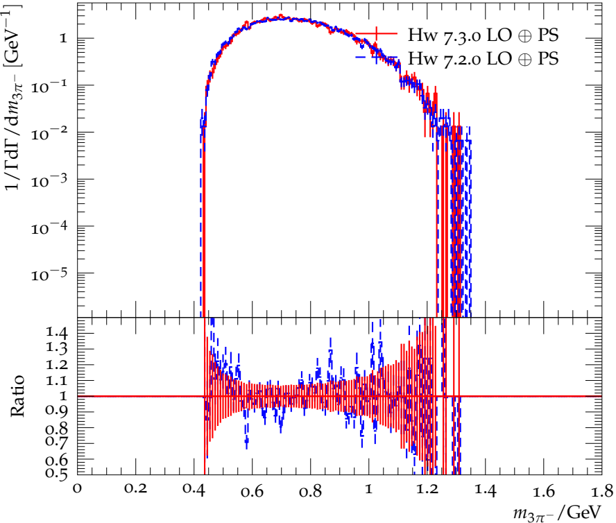
Distribution of the 3\pi^- mass for \tau^- \rightarrow 3\pi^- 2\pi^+ \nu_\tau
