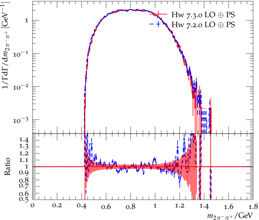
Distribution of the 2\pi^-\pi^+ mass for \tau^- \rightarrow 3\pi^-\pi^+\nu_\tau
