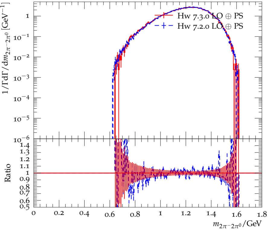
Distribution of the 2\pi^-2\pi^0 mass for \tau^- \rightarrow 2\pi^0 2\pi^- \pi^+ \nu_\tau
