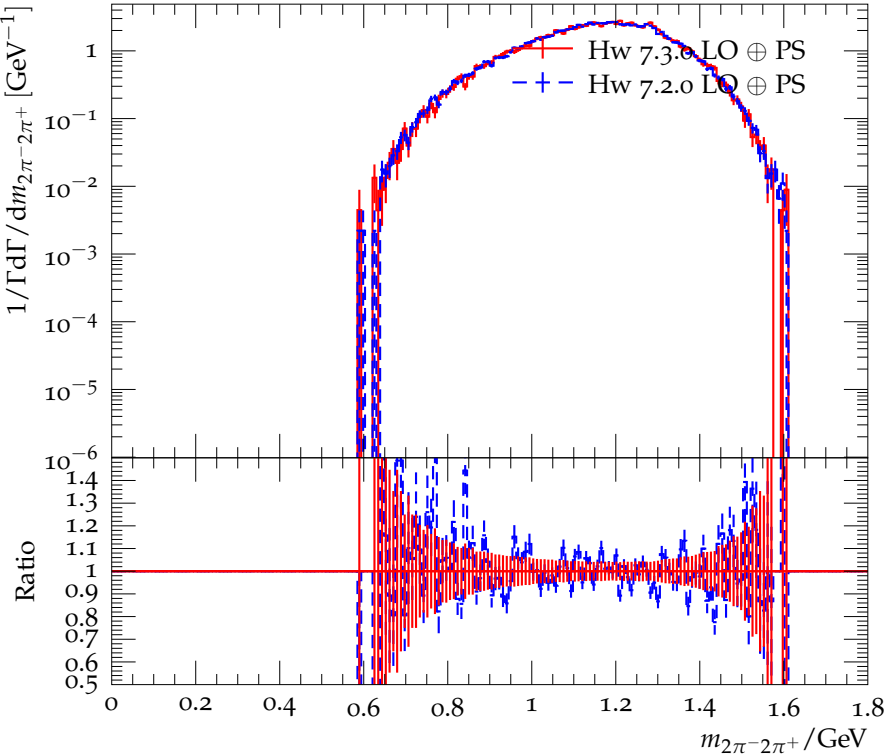
Distribution of the 2\pi^-2\pi^+ mass for \tau^- \rightarrow 3\pi^-2\pi^+\nu_\tau
