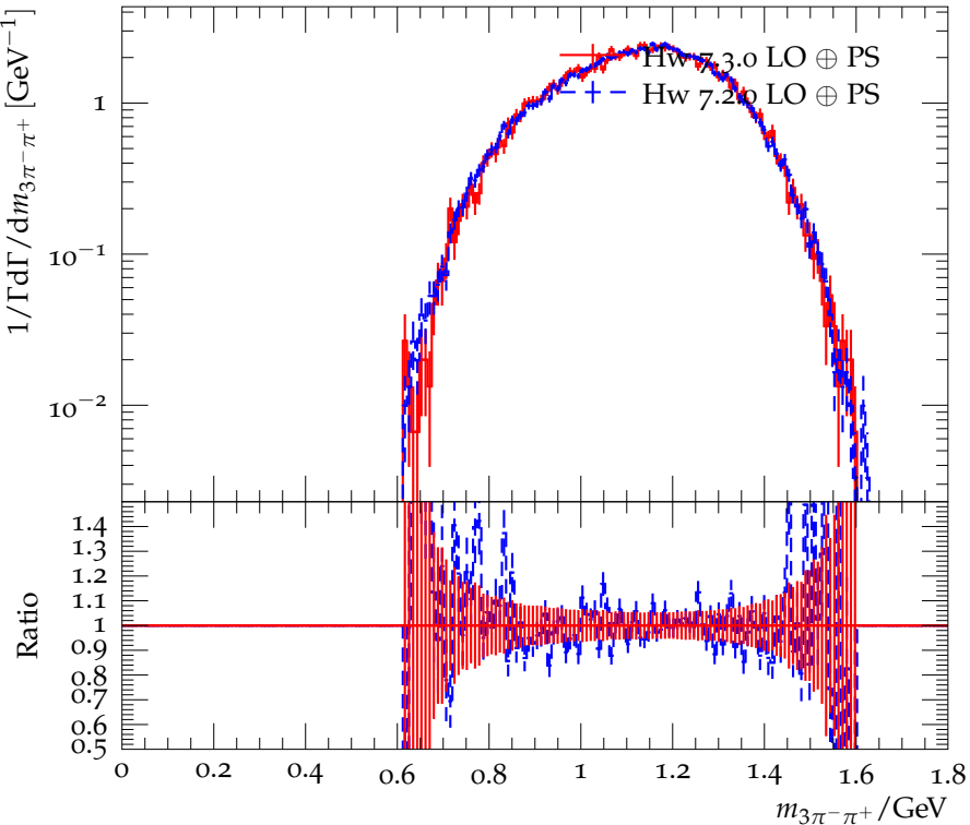
Distribution of the 3\pi^-\pi^+ mass for \tau^- \rightarrow 3\pi^-\pi^+\nu_\tau
