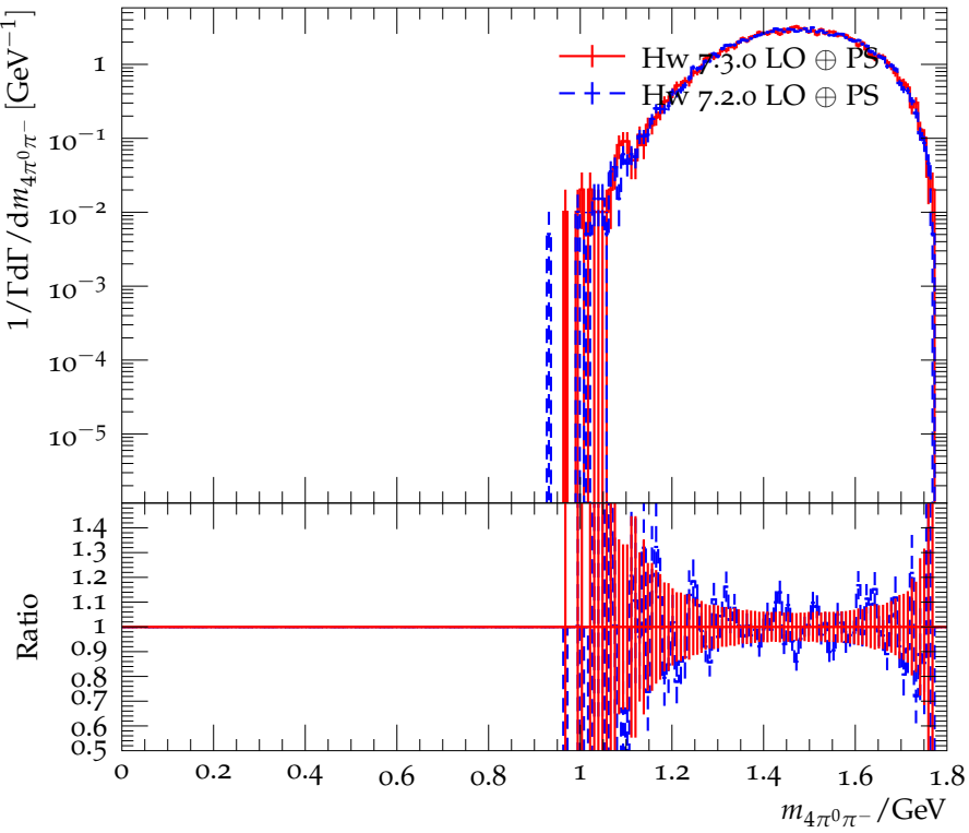
Mass distribution of the hadrons for \tau^- \rightarrow 4\pi^0 \pi^- \nu_\tau
