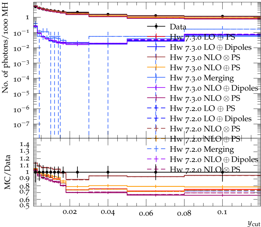
Number of photon vs y_{\text{cut}} , Durham
