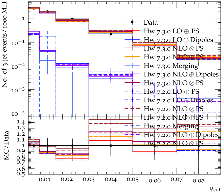
Number of 3 jet events vs y_{cut} , Jade
