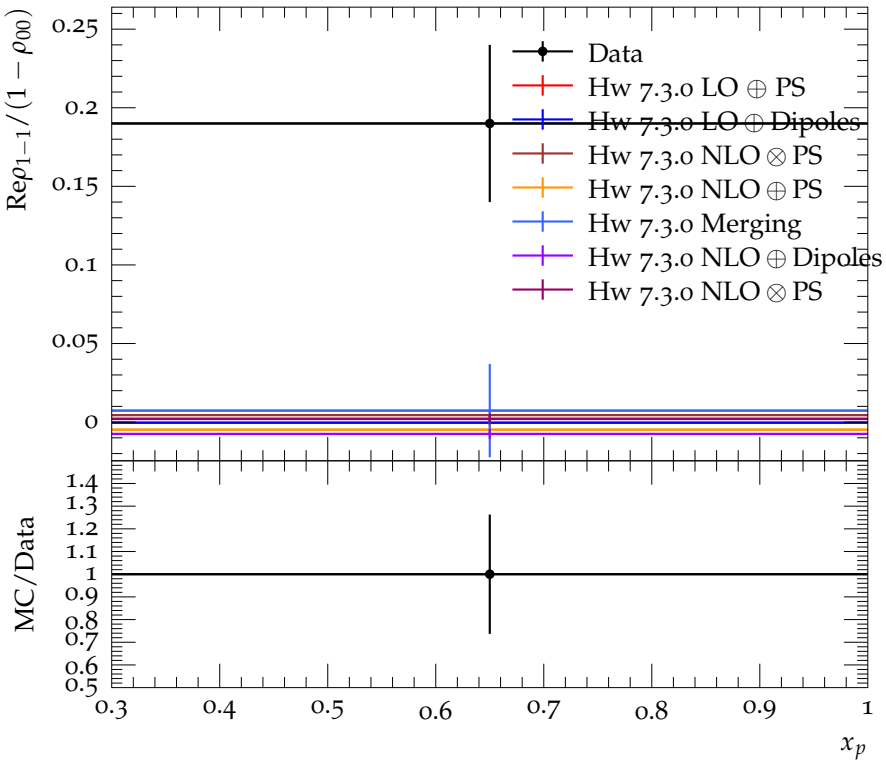
Ratio \text{Re}\rho_{1-1}/(1 - \rho_{00}) for x_p > 0.3
